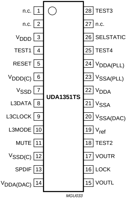
Fig.2 Pin configuration.
