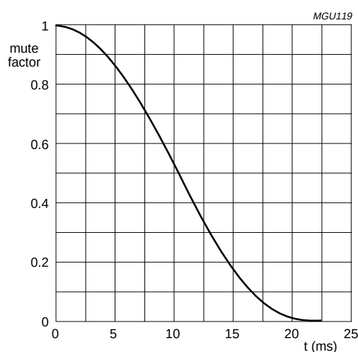
Fig.4 Mute as a function of raised cosine roll-off.
