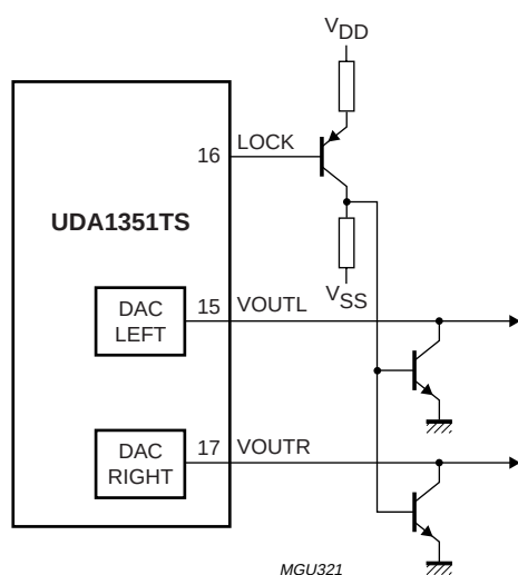
Fig.3 Example of external analog mute circuit.
